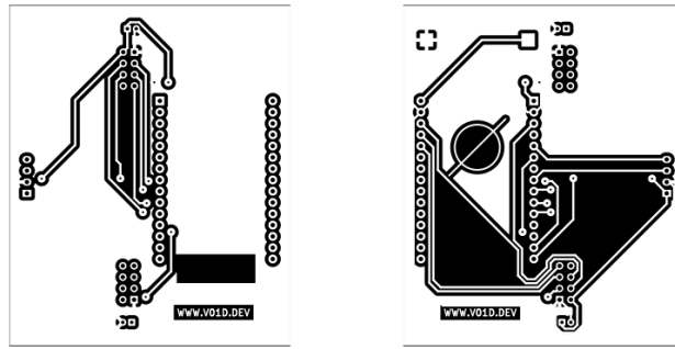
Front and back copper layers, exported from KiCad. These are the etch artwork.
